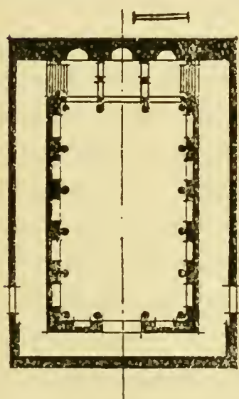
FIG. 62. Temple of Diana at Nîmes.
